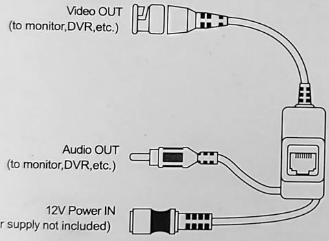
Injector
